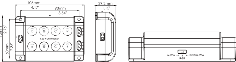
Dimensions (Unit: mm/inch)
