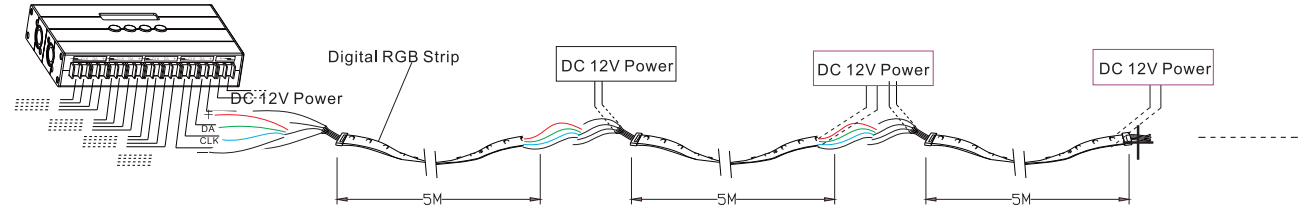
Connection Diagram
