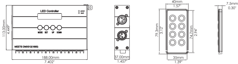
Dimensions (Unit: mm/inch)
