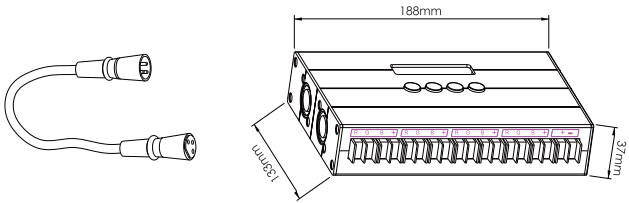
Dimensions (Unit: mm/inch)
