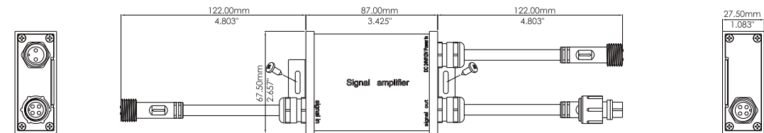
Dimensions (Unit: mm/inch)
