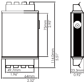
Dimensions (Unit: mm/inch)
