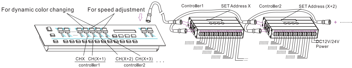
Connection Diagram
